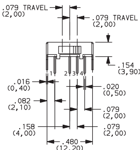
OS103011MA7QP1 SP3T
