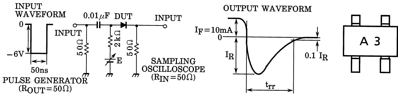
Fig.1 Reverse Recovery Time ( t_{rr} ) Test Circuit
