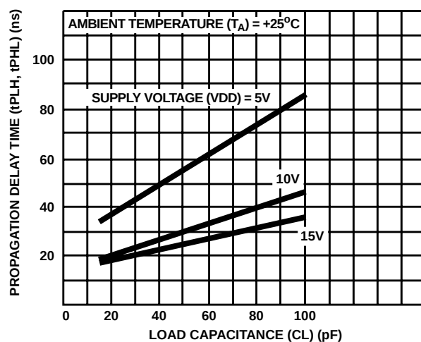
FIGURE 9. TYPICAL PROPAGATION DELAY TIME vs LOAD CAPACITANCE
