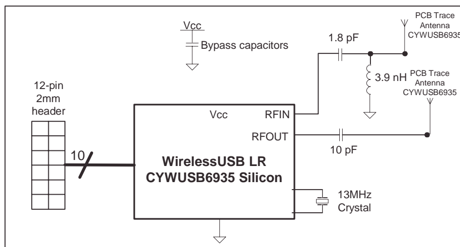
Figure 3-1. CYWM6935 Module
