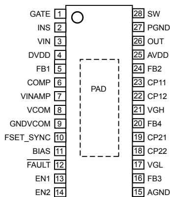
Pin-out Diagram
