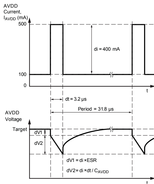
Figure 14. AVDD output voltage transient caused by a step change in load current
