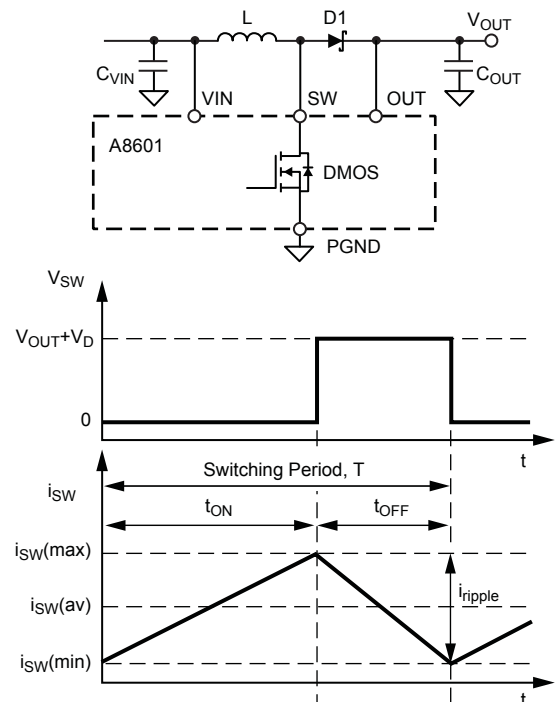
Figure 9. Continuous and discontinuous conduction mode factors
