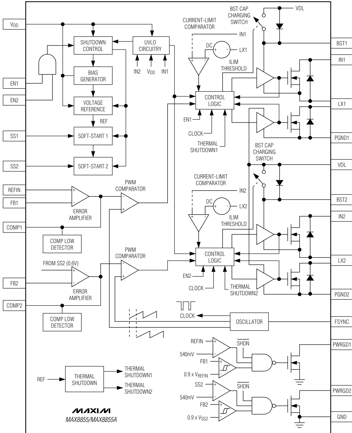
Figure 1. Functional Diagram
