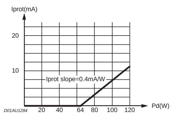
Figure 5. Protection current behaviour
