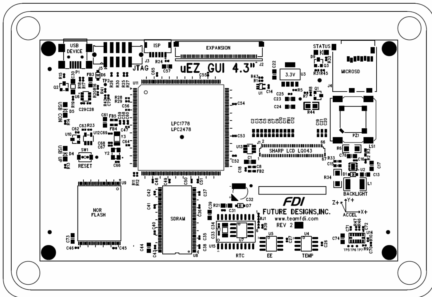
Figure 2 – uEZGUI-2478-43WQS Component View
