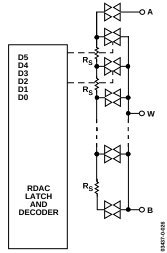
Figure 31. AD5171 Equivalent RDAC Circuit
