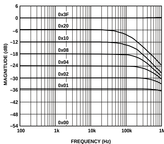
Figure 16. Gain vs. Frequency vs. Code, R_{AB} = 50 \Omega
