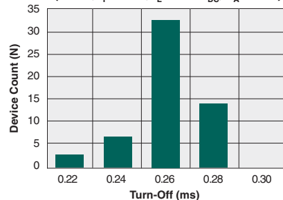
Typical Turn-Off Time (N=50, I_F=2\text{mA} , I_L=90\text{mA}_{DC} , T_A=25^\circ\text{C} )
