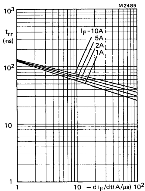
Fig.10 Maximum t_{rr} at T_j = 25\text{ }^{\circ}\text{C} ; per diode.
