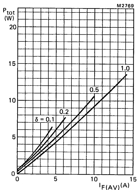
Fig. 5 Power rating per diode. The individual power loss in each diode should first be determined then both added together. The resulting total power loss is then used in conjunction with Fig.6 to determine the heatsink size and corresponding maximum ambient and mounting base temperatures.
