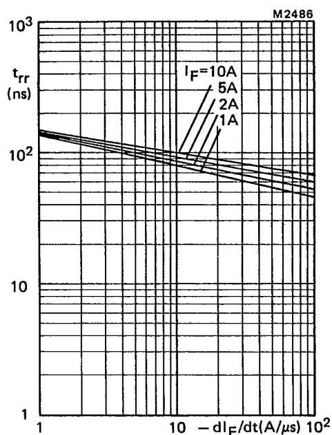
Fig.11 Maximum t_{rr} at T_j = 100\text{ }^{\circ}\text{C} ; per diode.
