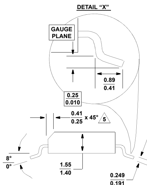
SIDE VIEW 2
