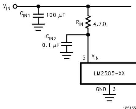
FIGURE 40. Input Line Filter
