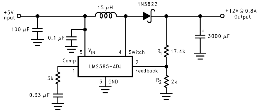
FIGURE 38. Boost Regulator
