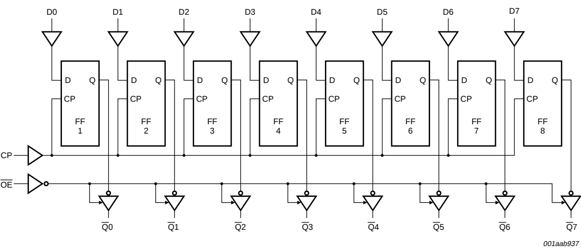
Fig 4. Logic diagram
