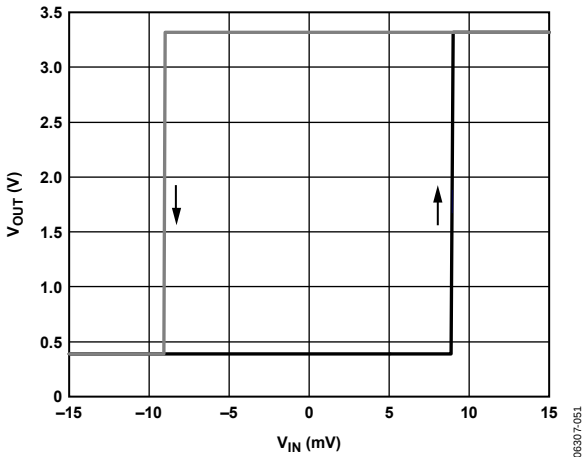
Figure 30. Comparator Hysteresis
