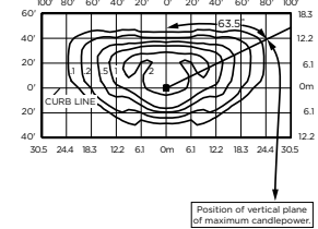
BXSPA*2HA-U Mounting Height: 25' (7.6m) Initial Delivered Lumens: 9,612 Initial FC at grade
