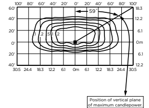
BXSPA*GHA-U Mounting Height: 25' (7.6m) A.F.G. Initial Delivered Lumens: 8,417 Initial FC at grade
