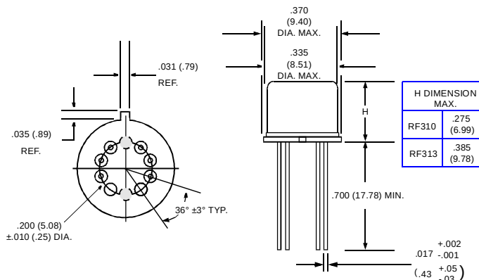
EXTERNAL DIMENSIONS
