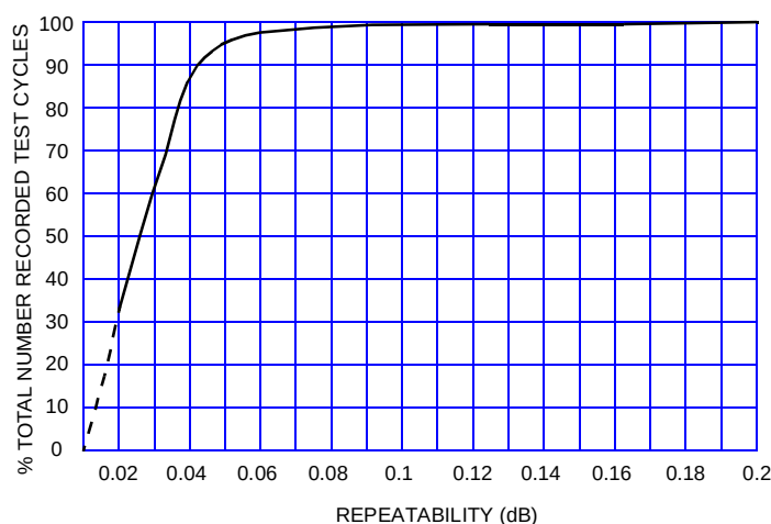
TYPICAL REPEATABILITY DATA, N.O. CONTACT
