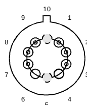
TERMINAL NUMBERING
