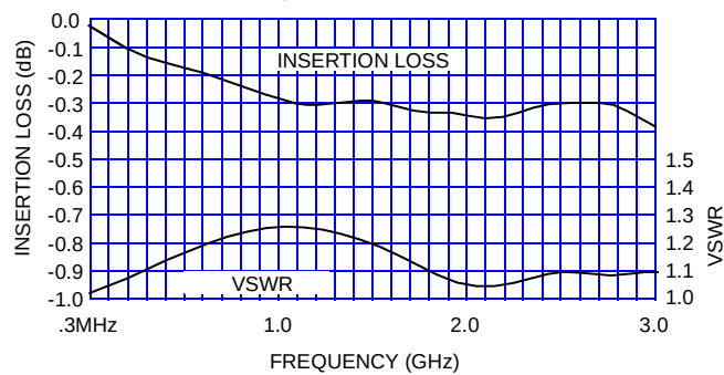
TYPICAL CHARACTERISTICS FOR N.C. BYPASS PATH, COIL DE-ENERGIZED
