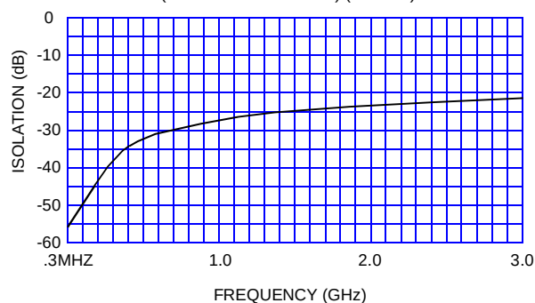
ISOLATION N.O. CONTACTS TO N.C. BYPASS PATH (COIL DE-ENERGIZED) (NOTE 6)
