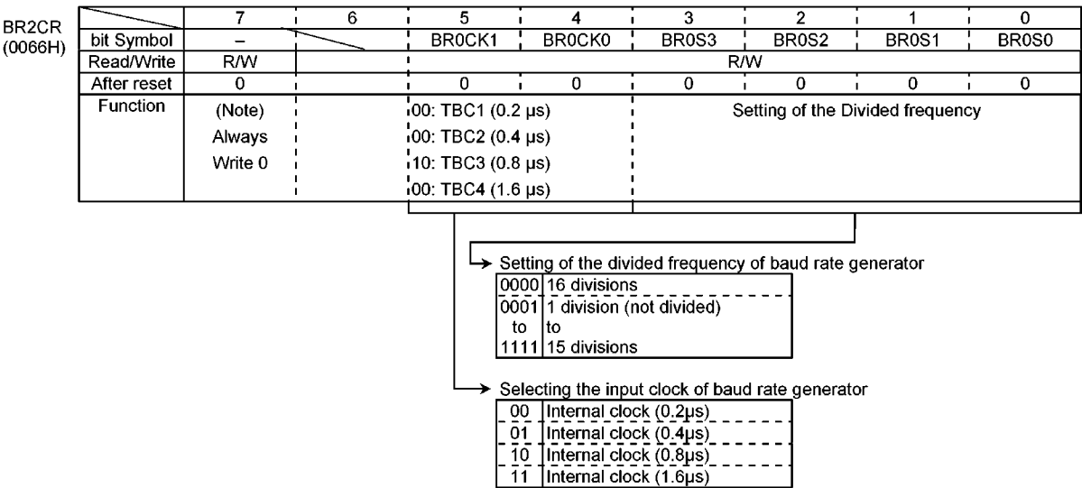
Figure 3.17.4 Serial Channel Control (BR2CR)
