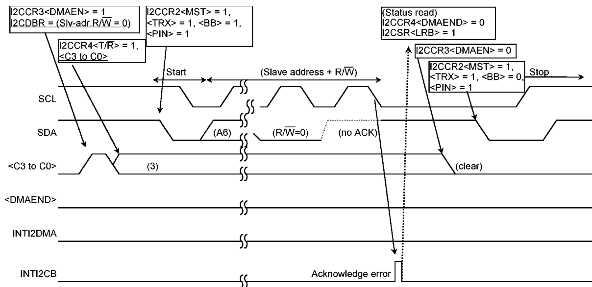
Figure 3.18.6-3 Example for the Acknowledge error at micro DMA transfer mode
