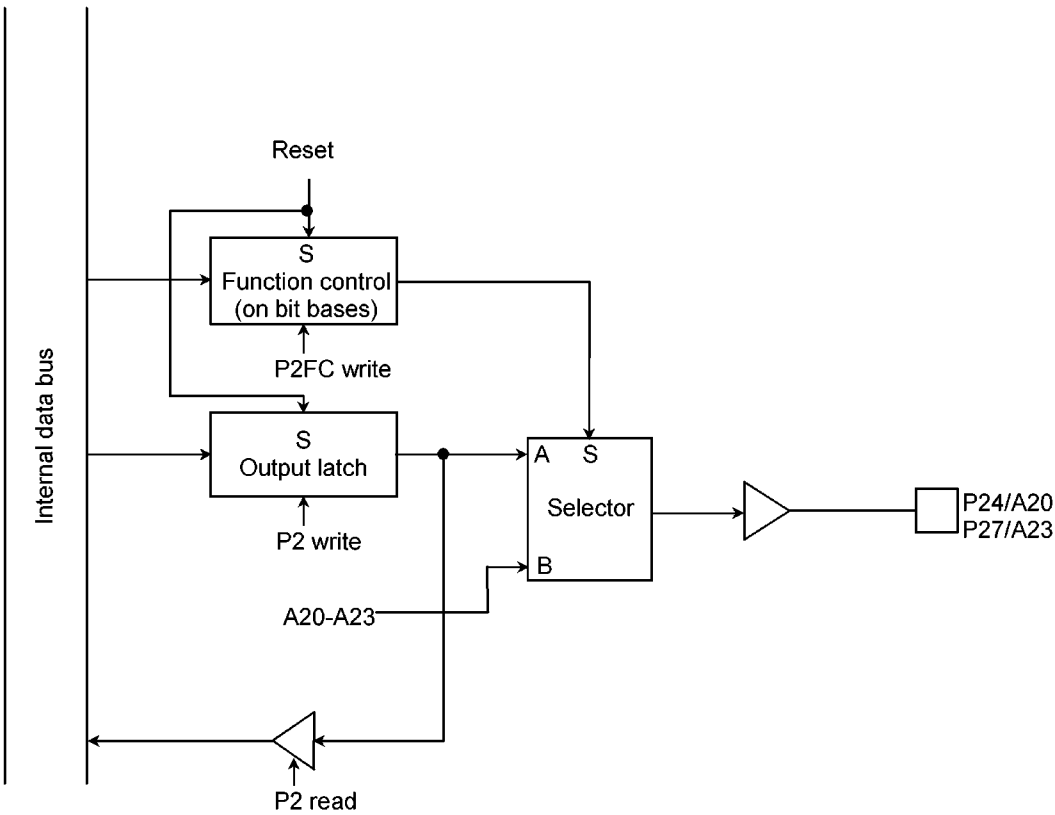
Figure 3.5.1 Port 2 (P24 to P27)
