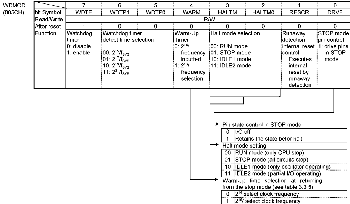
Figure 3.3.6 Watchdog timer mode register
