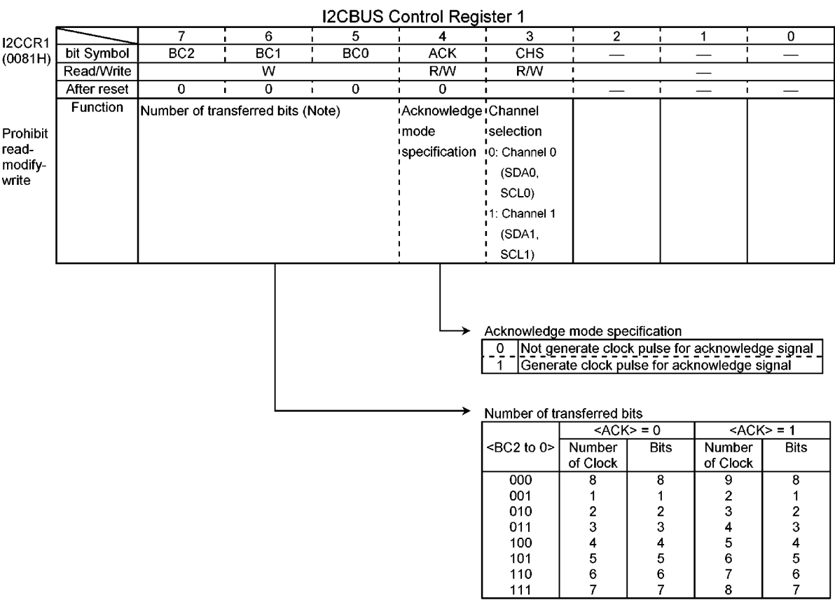
Figure 3.18.3 Register for I 2 C Bus
