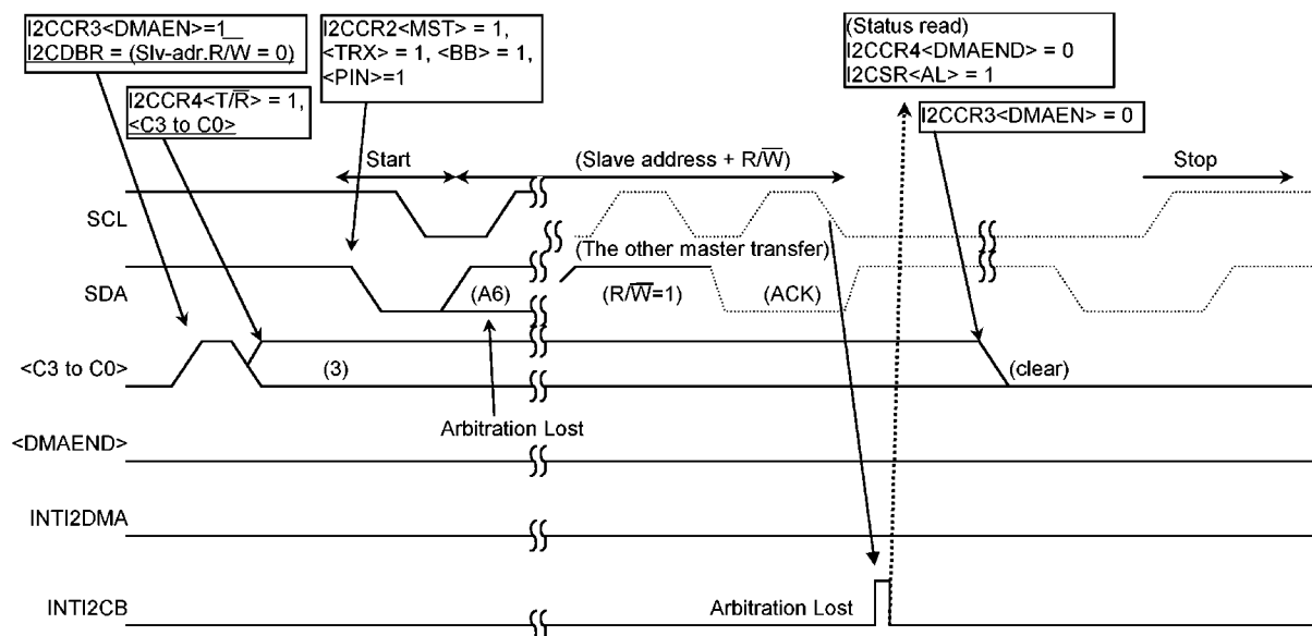
Figure 3.18.6-4 Example for the Arbitration lost at micro DMA transfer mode
