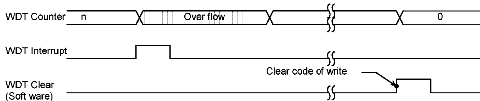
Figure 3.20.2 Normal Mode
