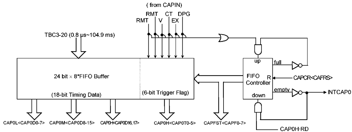
Figure 3.8.4 Structure of Capture 0
