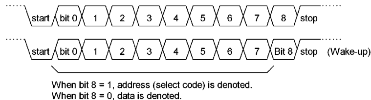
Figure 3.17.1 Data Formats
