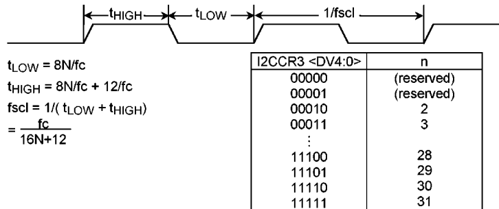
Figure 3.18.9 Clock Source
