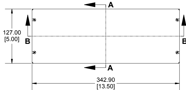
Bottom View of Assembly
