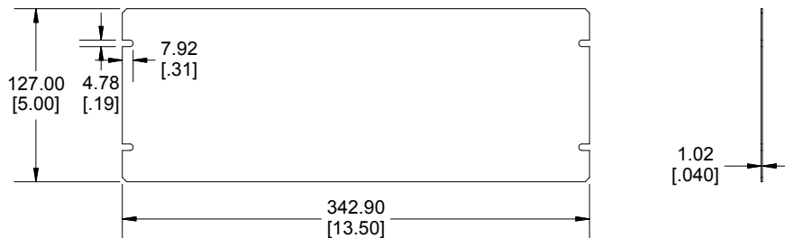
Bottom Plate (Sold Separately)
