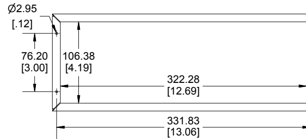
Bottom View of Chassis (Sold Separately)
