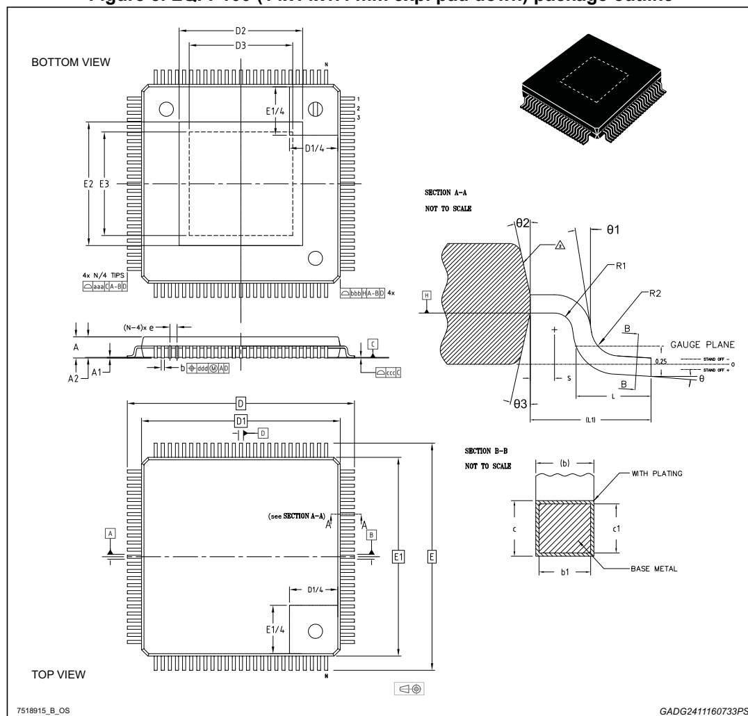
Figure 3. LQFP100 (14x14x1.4 mm exp. pad down) package outline
