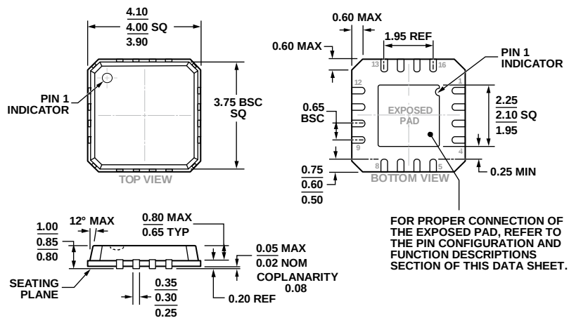
Figure 33. 16-Lead Lead Frame Chip Scale Package [LFCSP_VQ] 4 mm × 4 mm Body, Very Thin Quad (CP-16-4)
