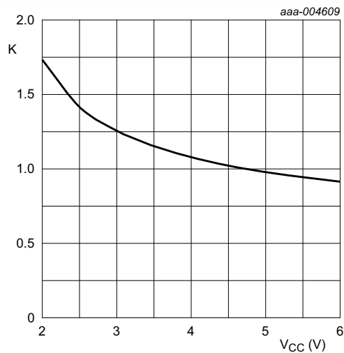
K-factor for 74HC132
