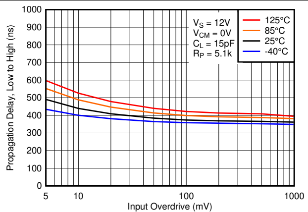
Figure 6-28. Low to High Propagation Delay vs. Input Overdrive Voltage, 12V
