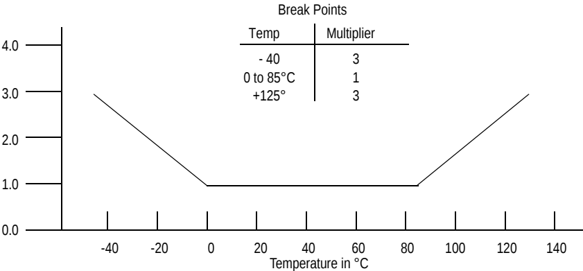
MPX5100D/MPX5100G/MPXV5100G Series
