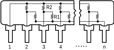
-5 Circuit Dual Terminator
