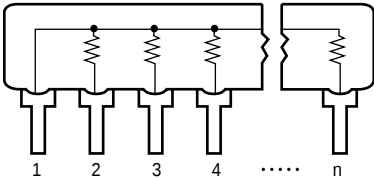
-1 Circuit Bussed Resistors
