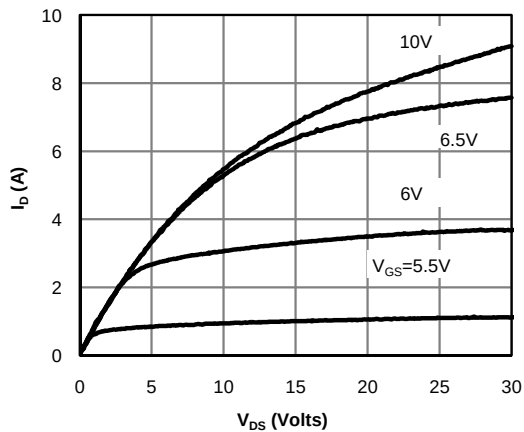
Fig 1: On-Region Characteristics
