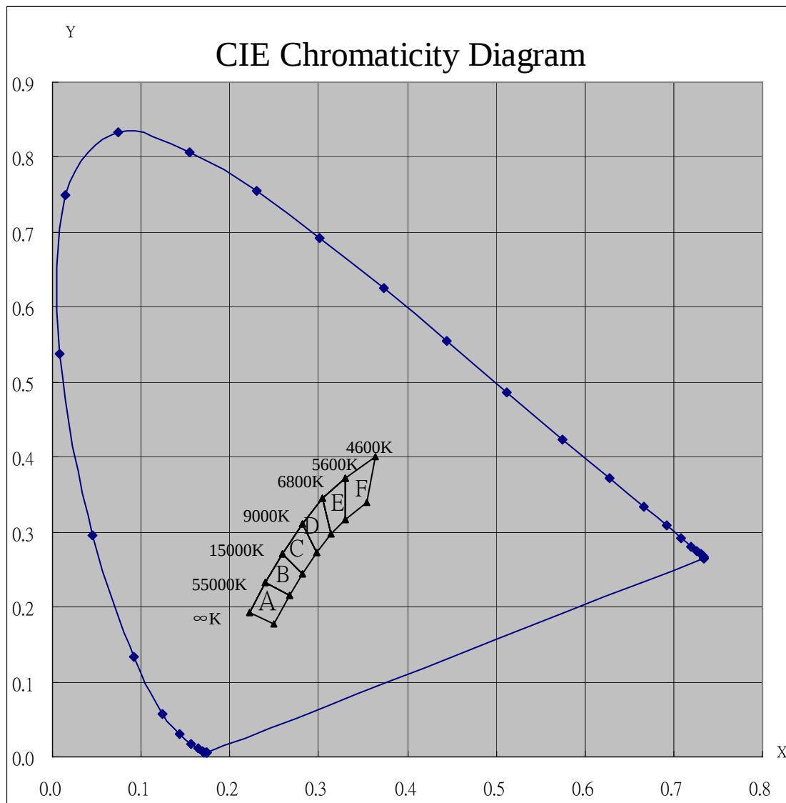
Color Ranks(IF=20mA,Ta=25℃)
