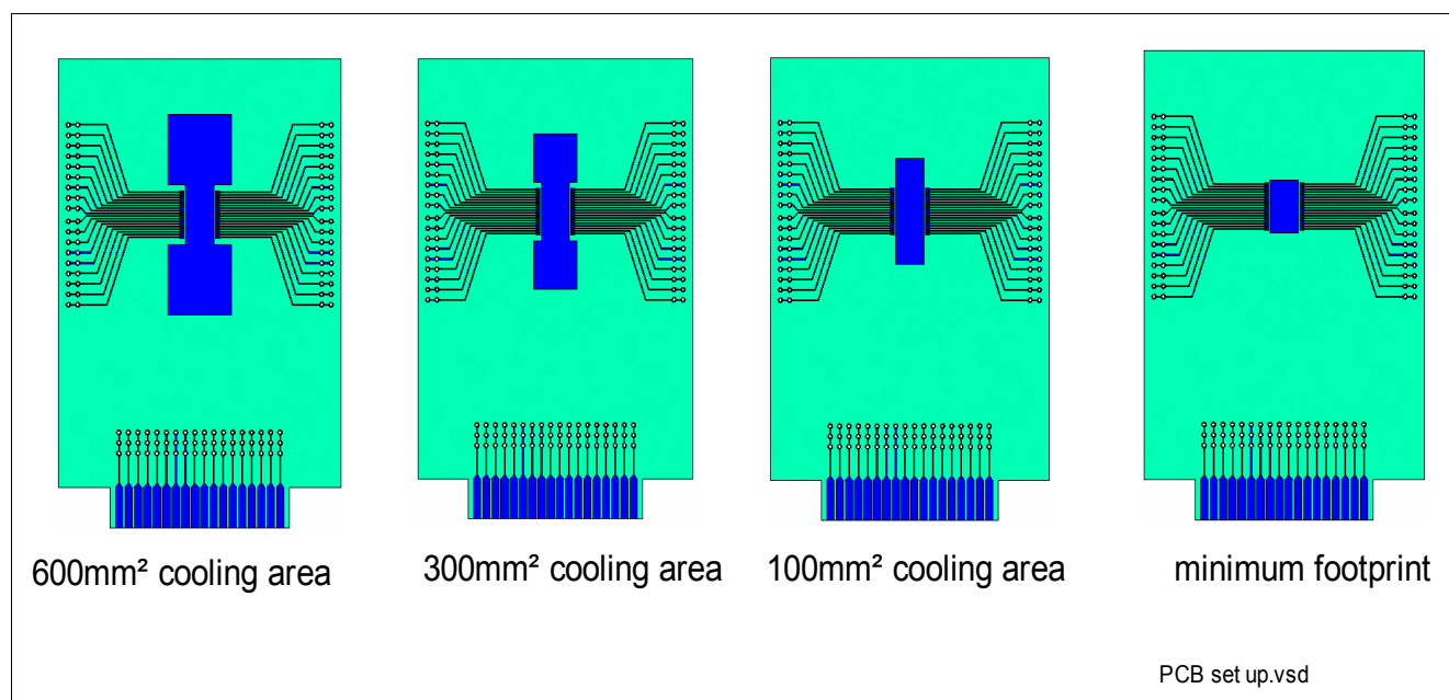
Figure 50 Board Set-up
