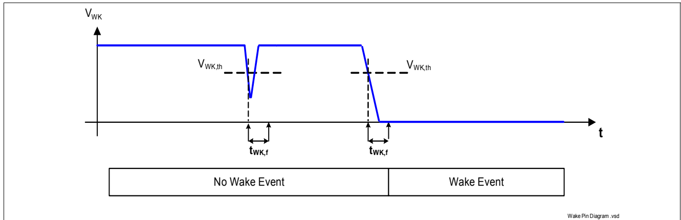
Figure 19 Wake-up Timing
