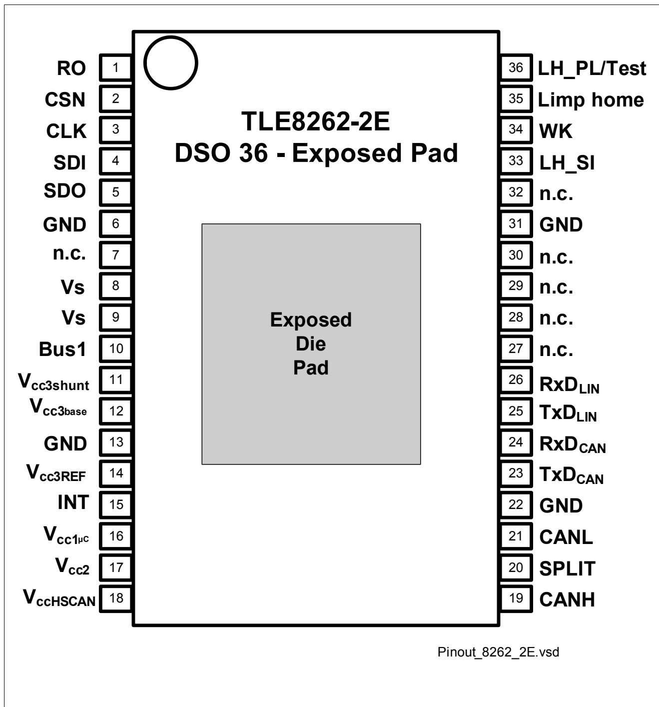
Figure 4 Pin Configuration
