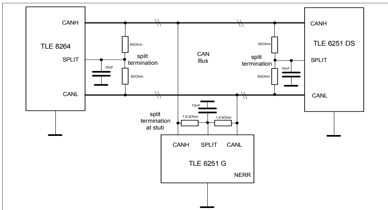
Figure 16 Application example for the SPLIT Pin
