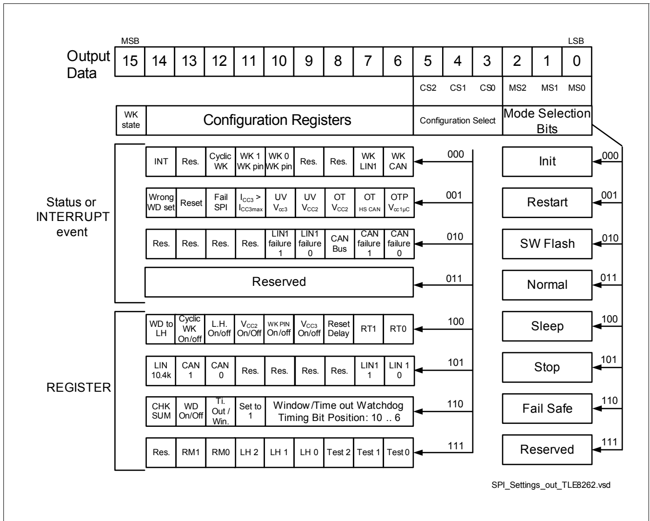
Figure 42 16-bit SPI Output Data / Control Word
