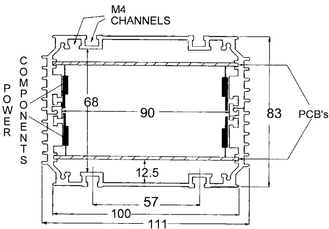
Figure 1: HSK Heatsink with dimensions (mm)
