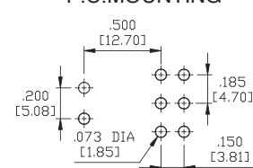
P.C.MOUNTING
