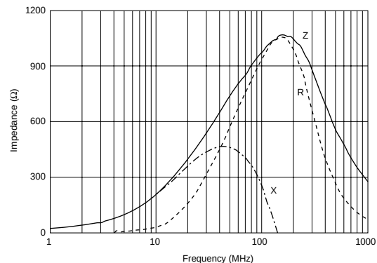
BLM15AG102SN1
