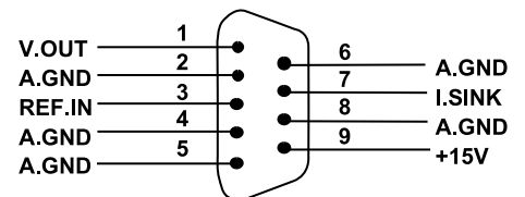
Pin Assignments for the DB-9 Connector
