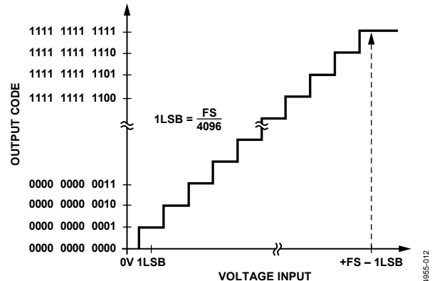
Figure 38. ADC Transfer Function in Pseudo Differential or Single-Ended Mode
