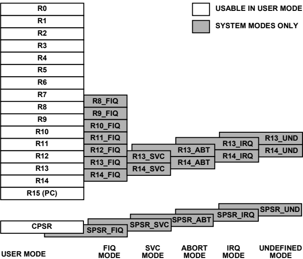
Figure 33. Register Organization
