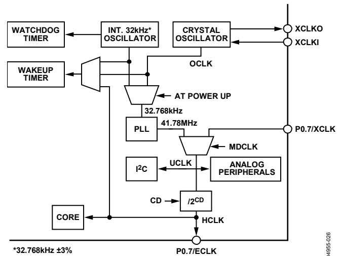
Figure 56. Clocking System
