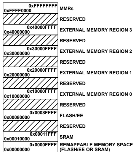
Figure 34. Physical Memory Map
