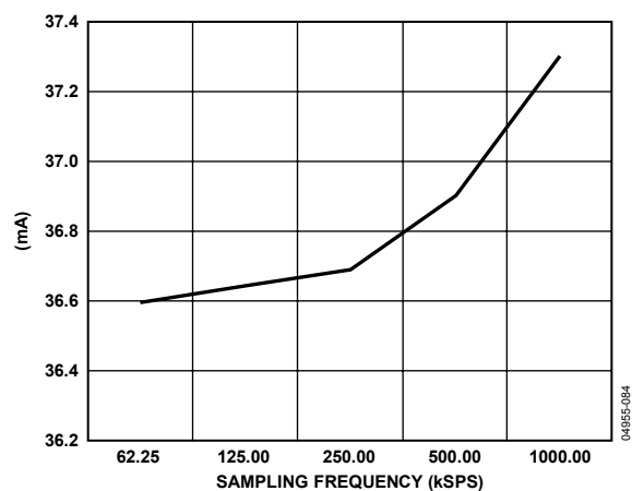
Figure 32. Current Consumption vs. Sampling Frequency
