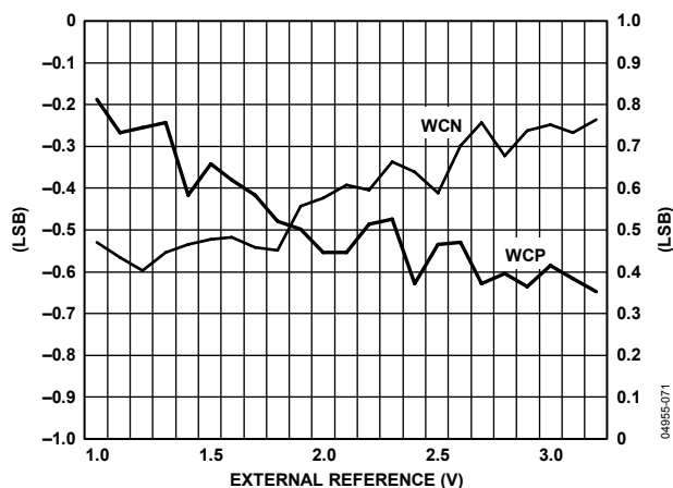
Figure 22. Typical Worst-Case DNL Error vs. V_{REF} , f_S = 774 kSPS
