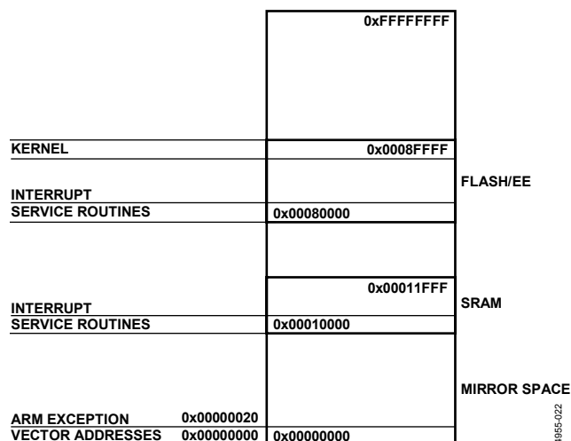
Figure 51. Remap for Exception Execution
