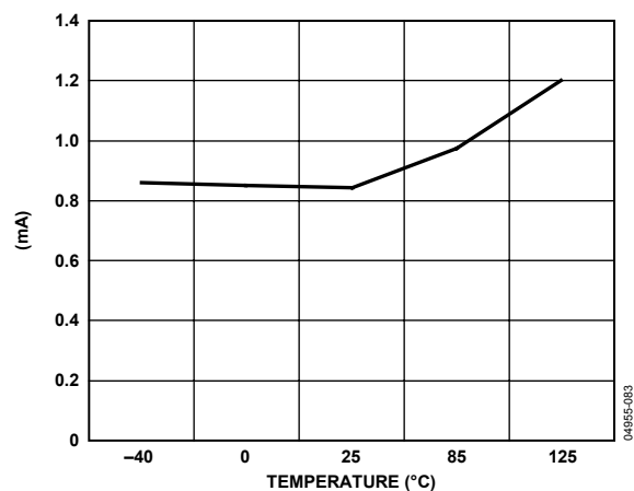
Figure 31. Current Consumption vs. Temperature in Sleep Mode
