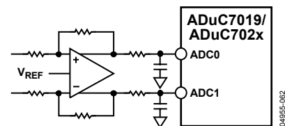
Figure 49. Buffering Differential Inputs
