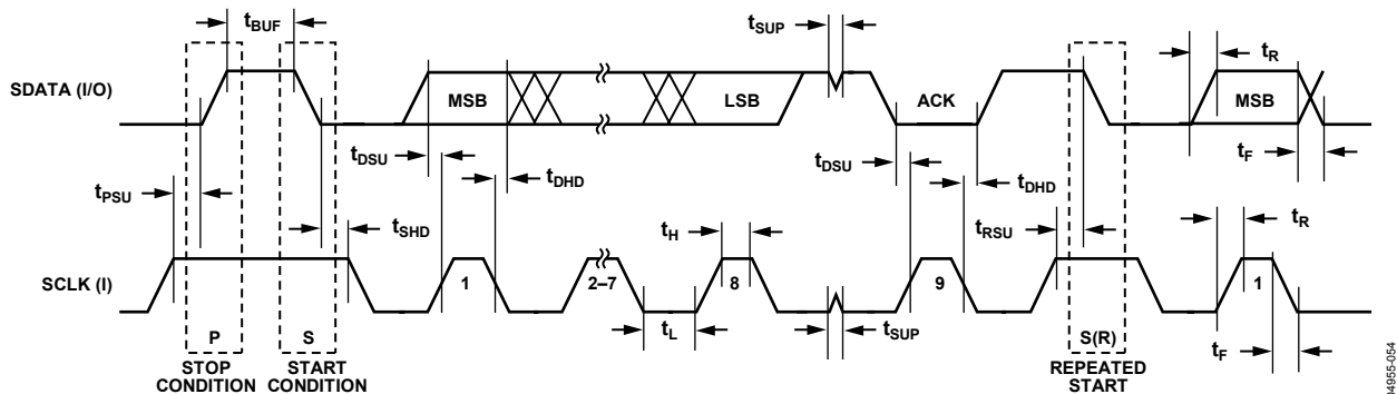
Figure 5. I 2 C Compatible Interface Timing
