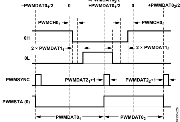
Figure 59. Typical PWM Outputs of the 3-Phase Timing Unit (Double Update Mode)
