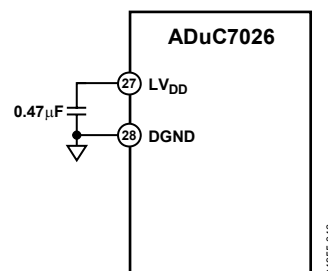
Figure 77. Voltage Regulator Connections
