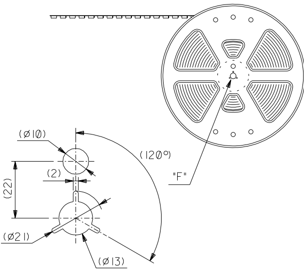
DETAIL "F"
