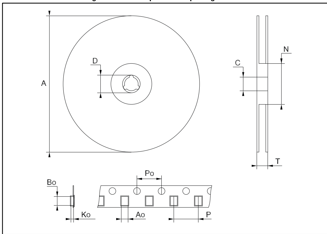
Figure 15: SO16 tape and reel package outline
