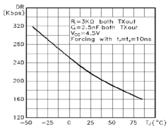
Figure 4: Data rate vs temperature
