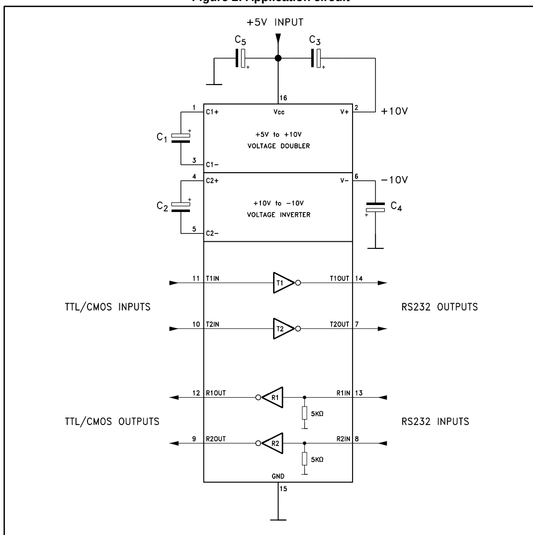
Figure 2: Application circuit
