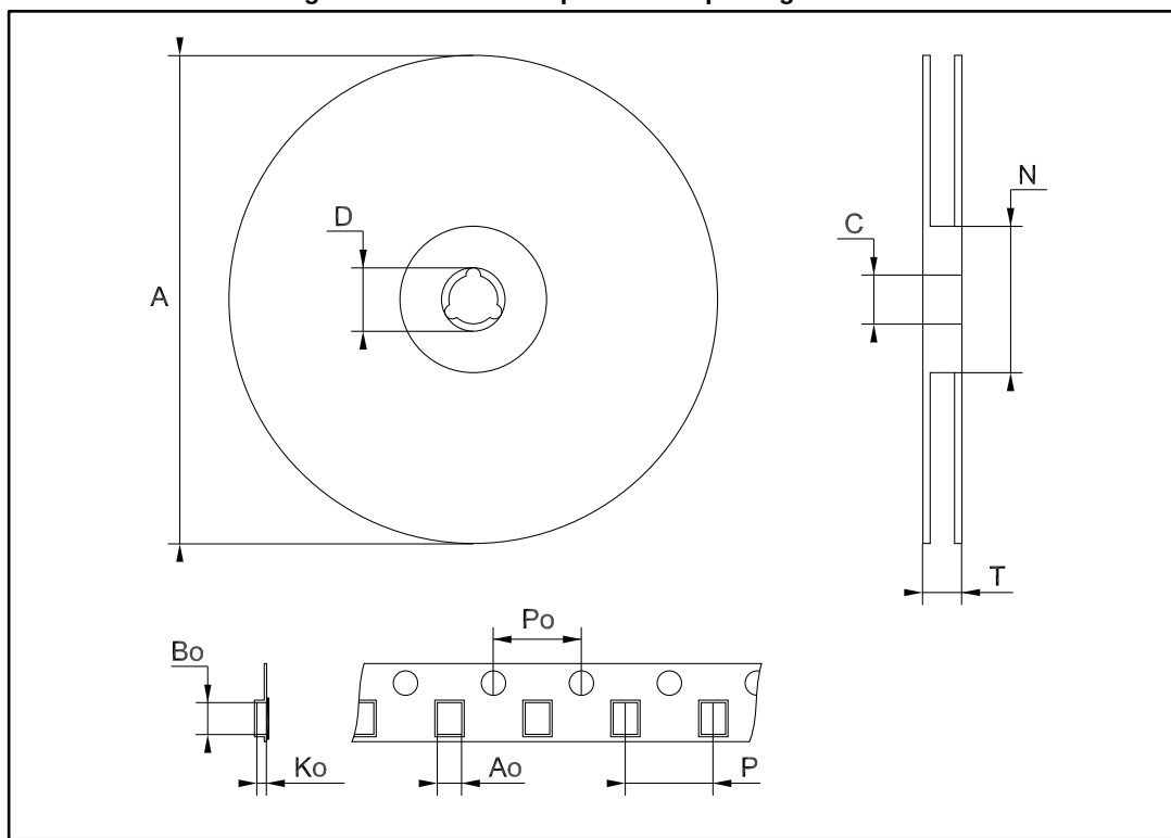
Figure 16: TSSOP16 tape and reel package outline
