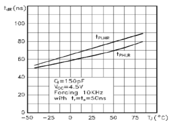
Figure 5: Receiver propagation delay
