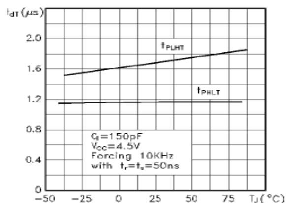
Figure 6: Driver propagation delay
