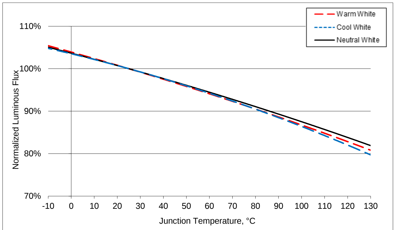
Figure 3: Typical Flux vs. Junction Temperature
