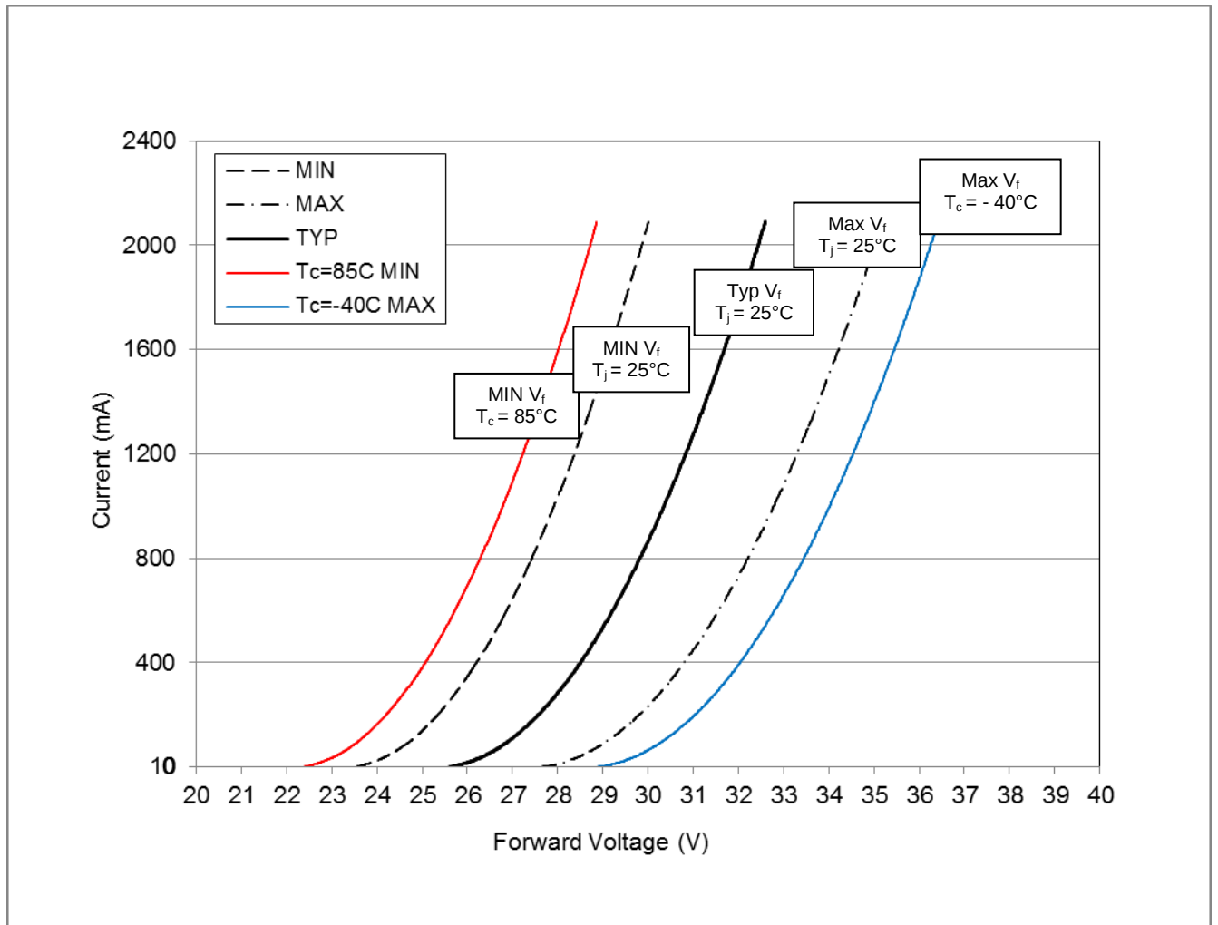
Figure 1: Electrical Characteristics
