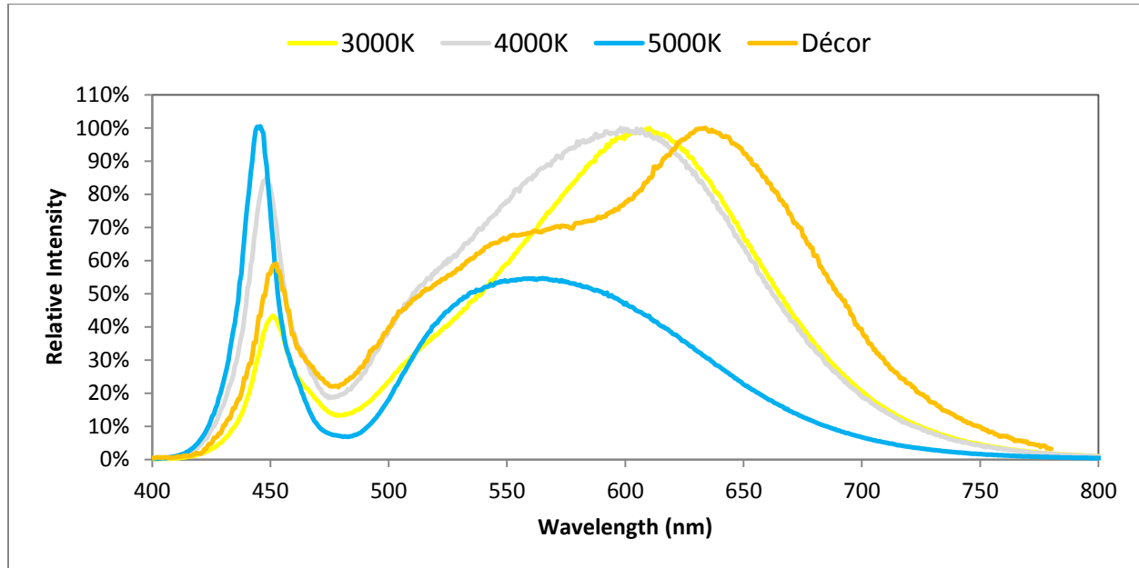
Figure 8: Typical Color Spectrum
