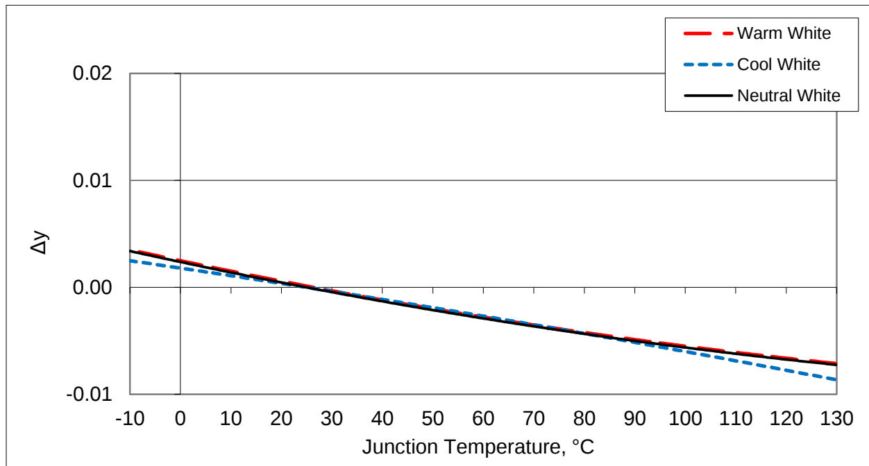
Figure 4: Typical ccy Shift vs. Junction Temperature
