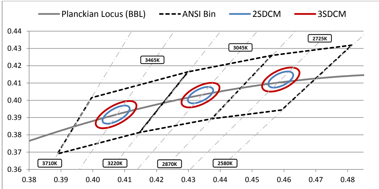
Figure 10: Graph of Warm White Test Bins in xy Color Space
