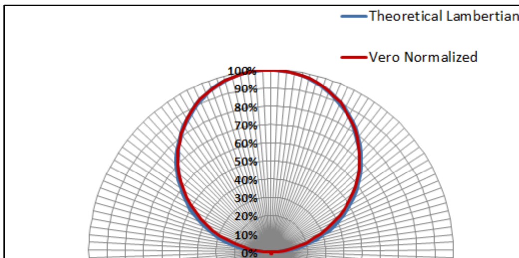
Figure 7: Typical Polar Radiation Pattern
