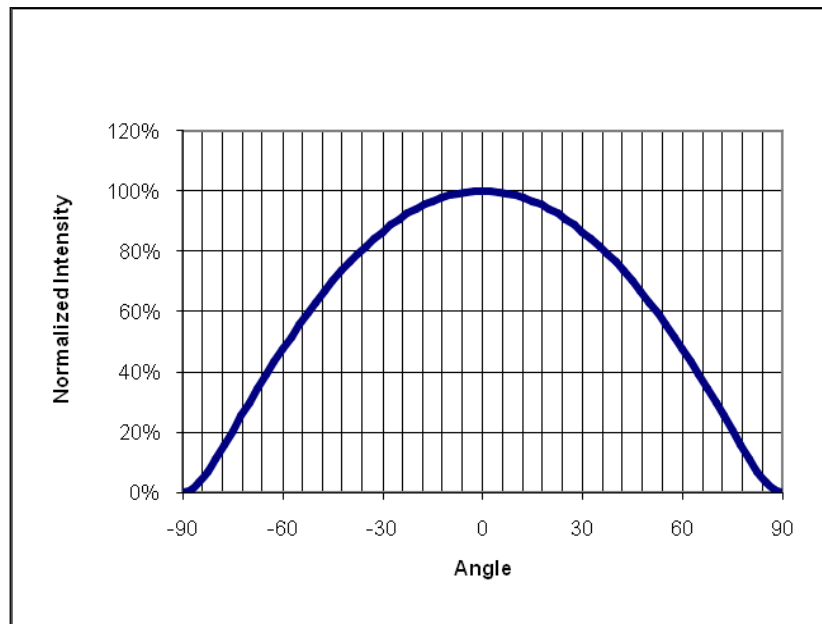
Figure 6: Typical Spatial Radiation Pattern
