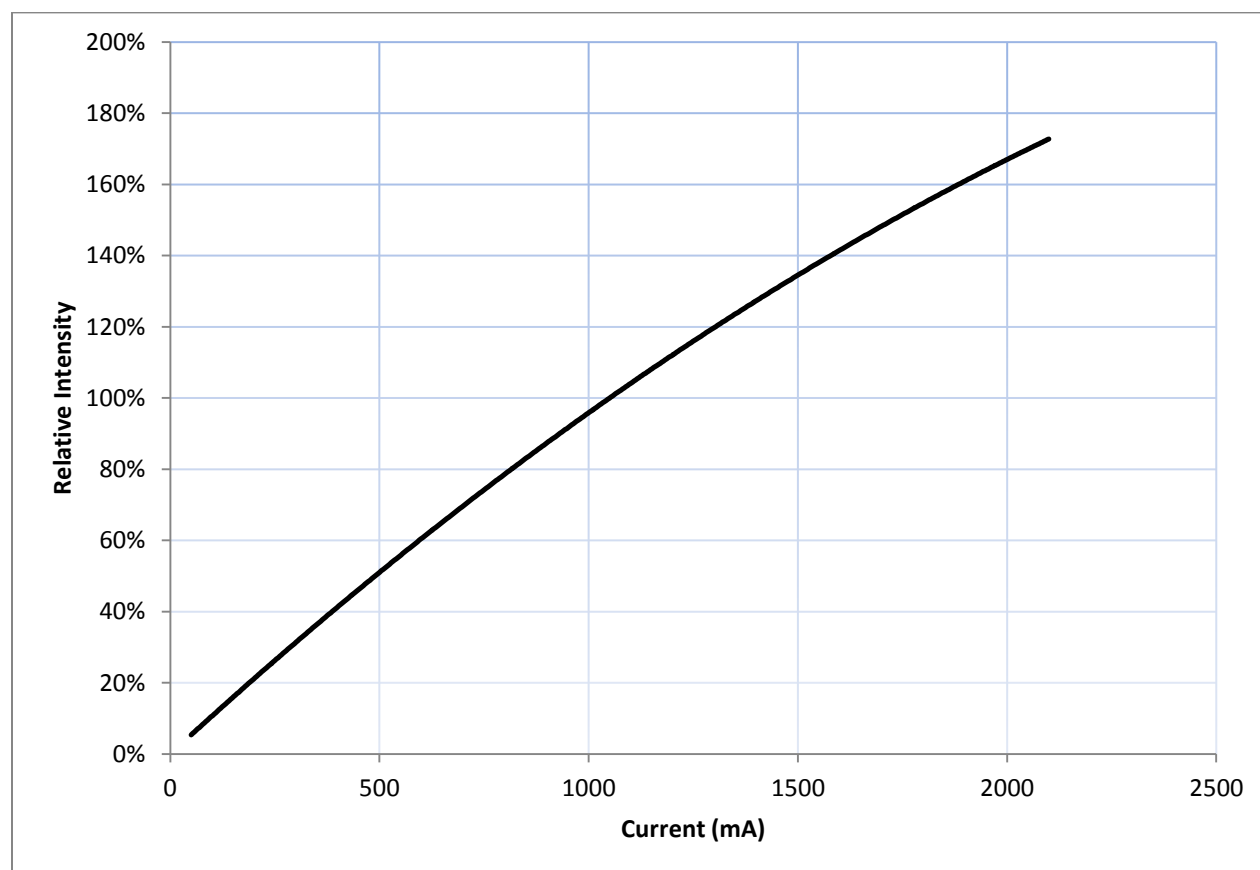
Figure 2: Typical Flux vs. Current, T_j = 25^{\circ}\text{C}
