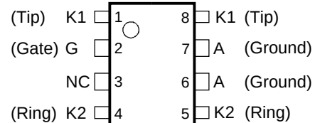
P PACKAGE (TOP VIEW)
