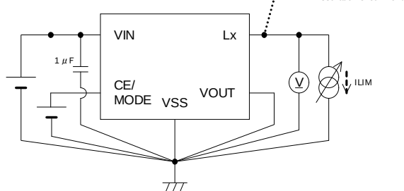
Circuit⑨
