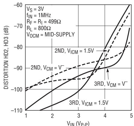
Differential Distortion vs Input Amplitude (Single-Ended Input)
