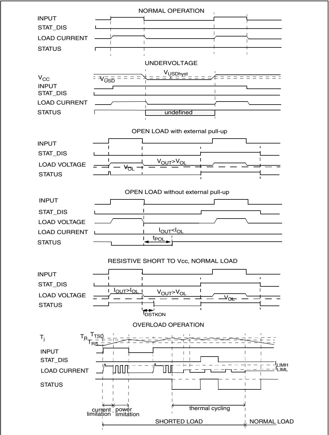
Figure 7. Waveforms
