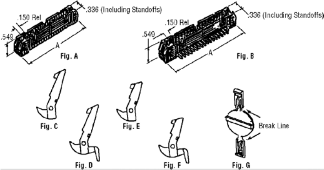
Military, Center and Dual Polarized; .100" × .100" Centers — Mate with Novo Receptacles — Terminate to PC Board
