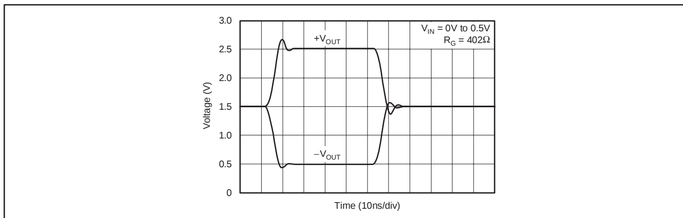
Figure 8. Pulse Response for Figure 7 Schematic
