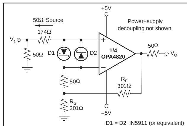
Figure 20. Gain of +2 with Input Protection
