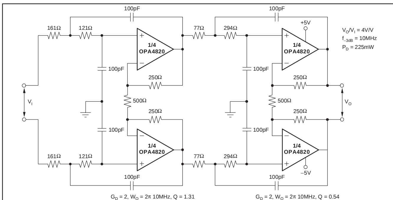
Figure 9. Low-Power, Differential I/O, 4th-Order Butterworth Active Filter
