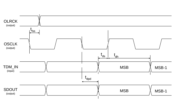
Figure 4. TDM Master Mode Timing
