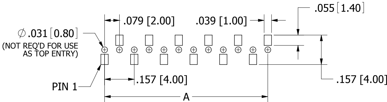
RECOMMENDED PCB LAYOUT SFM230-NPPN-S__-SD-BK
