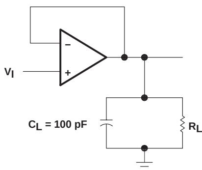
Figure 1. Unity-Gain Amplifier
