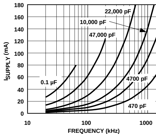
Supply Current vs. Frequency ( V_{DD} = 12V )
