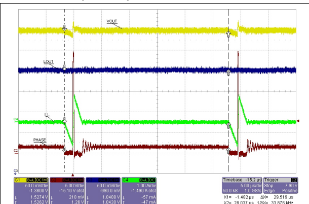
Figure 13. L_{OUT} turn on, V_{OUT} in pulse-skip mode
