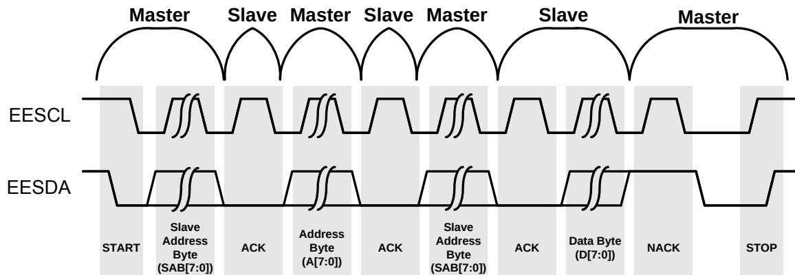
Figure 22.6. Selective Address Read (Single Byte)
