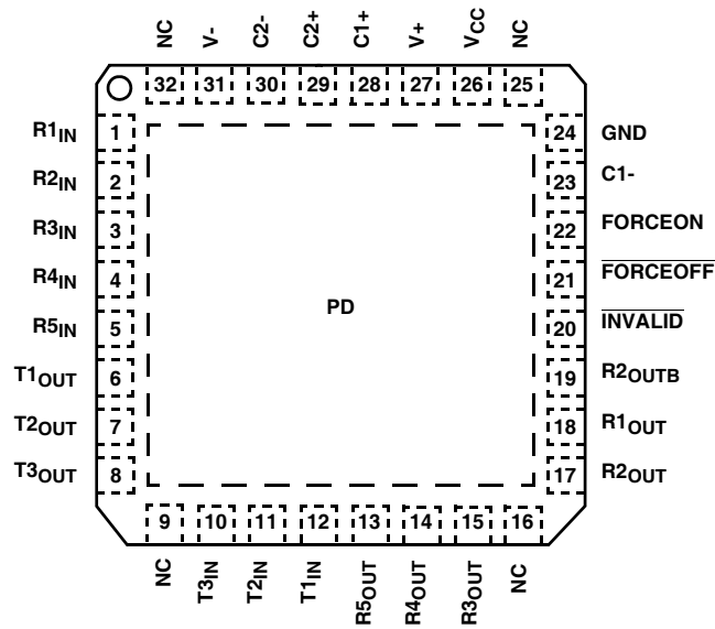
ISL4243E (32 LD QFN) TOP VIEW
