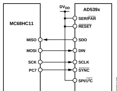
Figure 36. AD539x-MC68HC11 Interface
